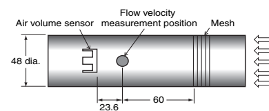
Figure 1: Wind Tunnel
