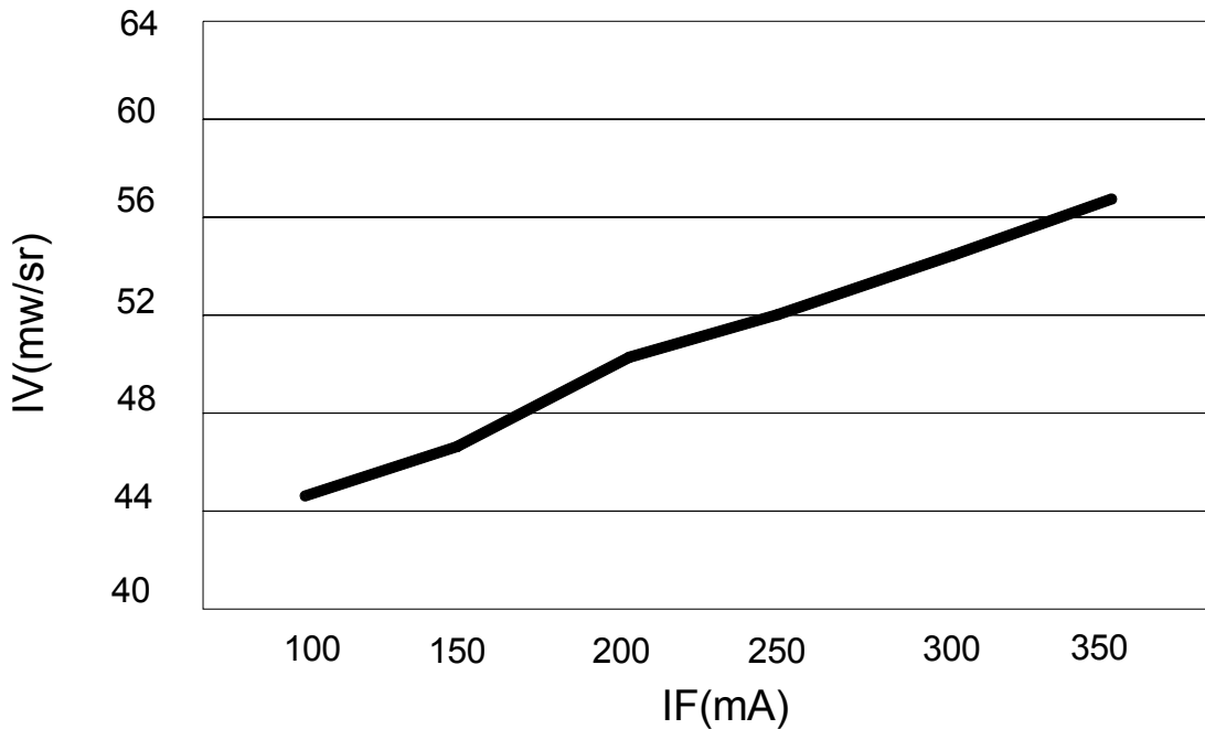
Forward Current & IV
