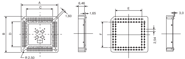
PLCC-xx
