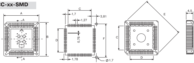
PLCC-xx
